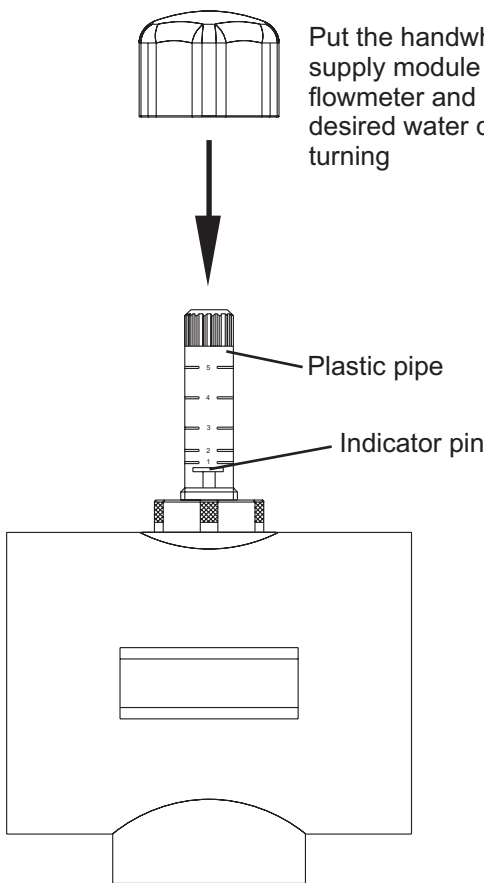
SBK Multipurpose manifold 5000 Return module with integrated flowmeter
